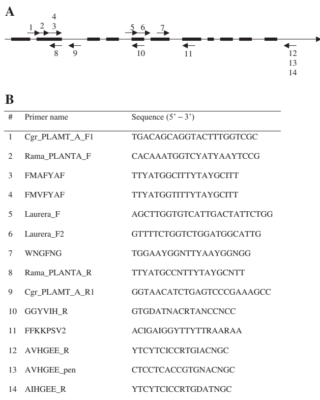
FIG. 1. Degenerate primers and priming sites. (A) Placement of degenerate primers relative to coding regions for transmembrane domains of Cladonia grayi mep1a (MEP \alpha clade, fig. 2). Transmembrane domains shown as thickened bars. Primers shown as numbered arrows. (B) Sequences of degenerate primers used to amplify “plant-like” MEP \alpha AMTPs from lichenized fungi (supplementary table S2, Supplementary Material online).
